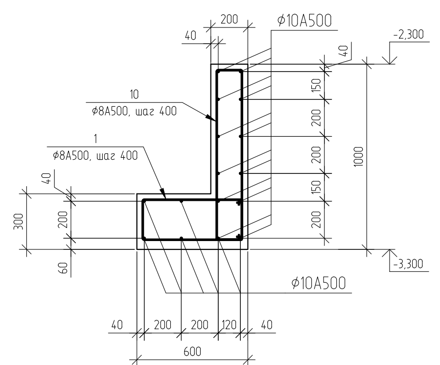
2-2
